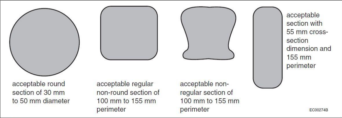
Figure A-9.8.7.5.(2) Handrail sections
