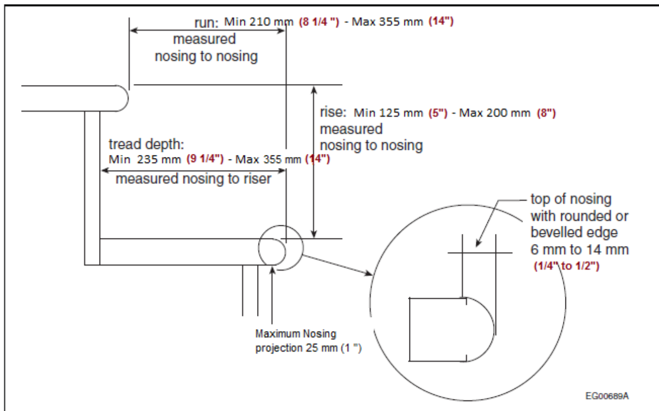
Figure A-9.8.4.-B Measurements shown are interior or exterior stairs serving (a) single dwelling units, (b) houses with a secondary suite or garages serving a or b Elements of steps and their measurement
